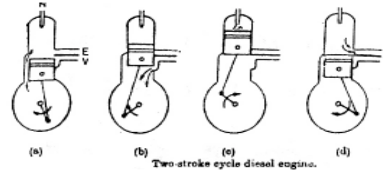
Two-stroke cycle diesel engine.
