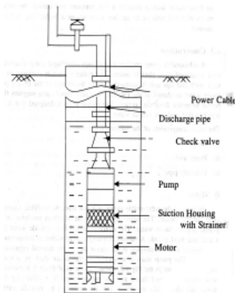
Fig 7.2 Line diagram of Submersible pump
