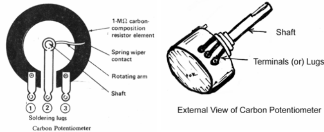
Fig.1.3 carbon potentiometer internal and external views
